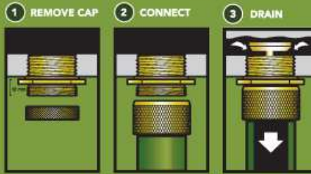
THREAD ON DRAINER: FOR EQUIPMENT WITH LIMITED SPACE OR LOW GROUND CLEARANCE
